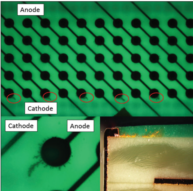
Figure 6-1 THB testing with 350 V at 85 °C, 85% rH; unexpected early failures due to anodic migration in the solder resist; anodic migration in the form of \text{Cu}_2(\text{OH})_3\text{Cl} or mixtures of \text{CuxO} identified [2, 3]
