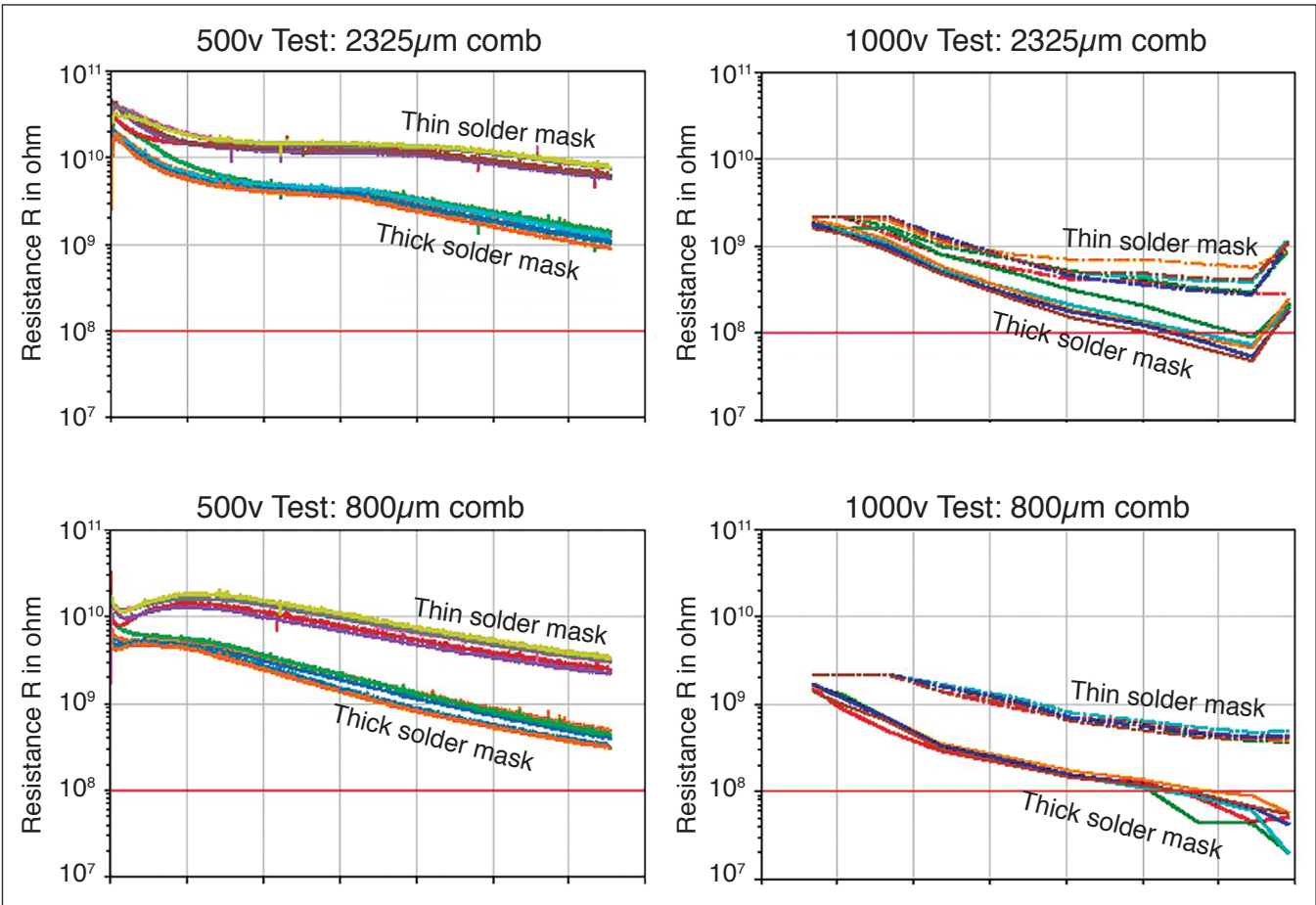
Figure 6-4 Insulation resistance measurement of printed boards with thin and thick applied solder mask tested at 85 °C, 85% rH. Insulation resistance is continuously decreasing without showing a clear drop indicating a failure. The decision criteria \text{Log} (\text{SIR} / (\text{Ohm})) < 8 as fail does not reflect the defects found by regular optical inspection during the test period [4]
