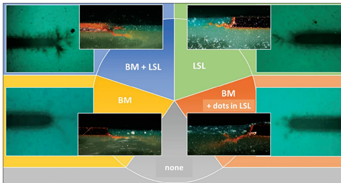
Figure 6-2 Top view in microscope with UV light and corresponding microsection of AMP failures; different propagation pathways are seen depending on solder resist (LSL) and base material (BM) [6]
