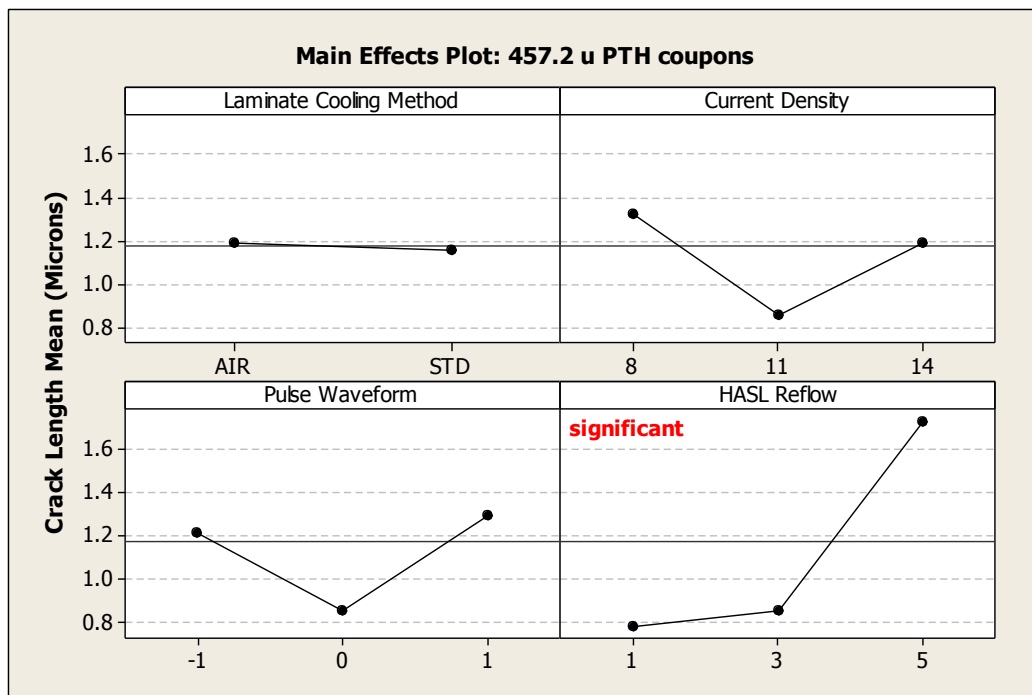
Figure 11 - Main Effects Plot: Maximum Crack Length (457.2 \mu m PTH coupons)
