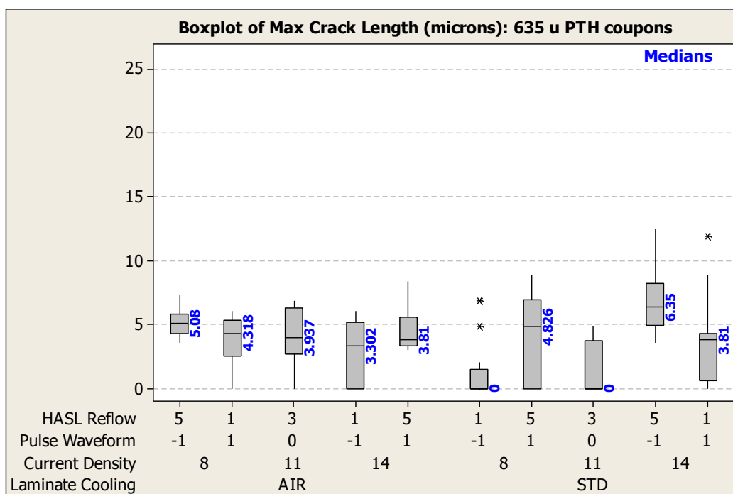
Figure 5: Box Plot of Maximum Crack Length (635 \mu\text{m} PTH coupons)
