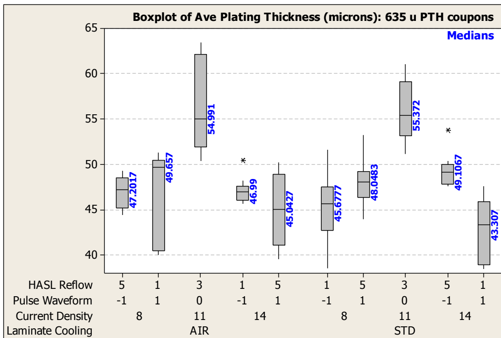
Figure 8 - Box Plot of Average Plating Thickness (635 \mu m PTH coupons)
