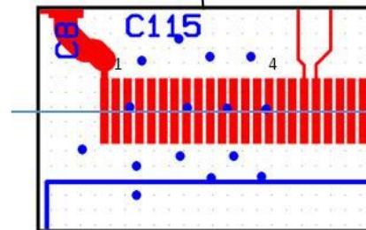
Coupon 3 (4 Locations- 381 \mu\text{m} (.015") BV3 Layers 2-15)
