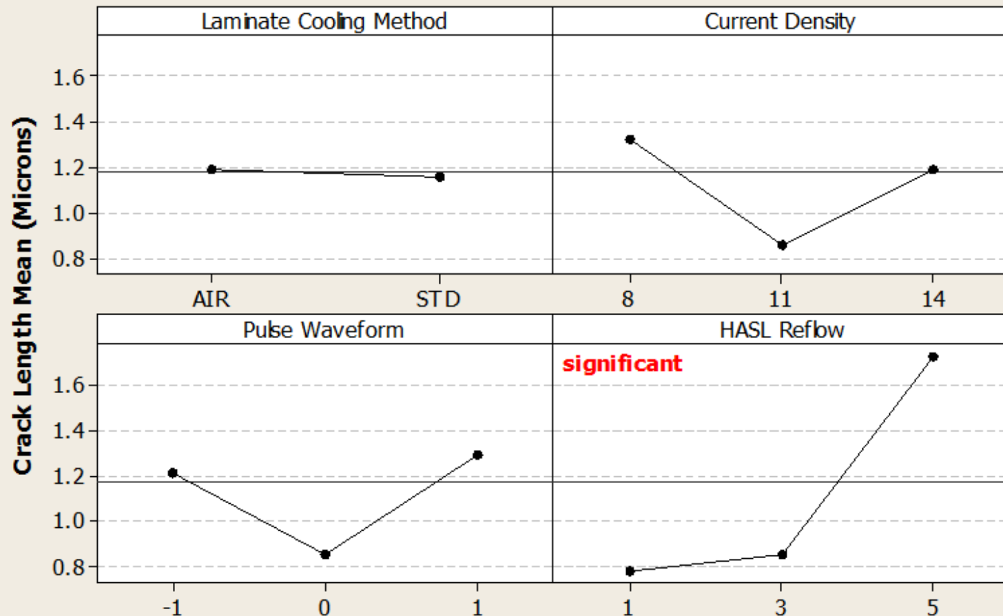
Main Effects Plot: 457.2 \mu\text{m} PTH coupons
