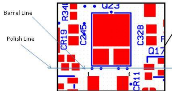
Coupon 2 (4 Locations- 457.2 \mu\text{m} (.018") PTH )
