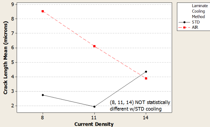
Interaction Plot for Max Crack Length: buried via coupons
