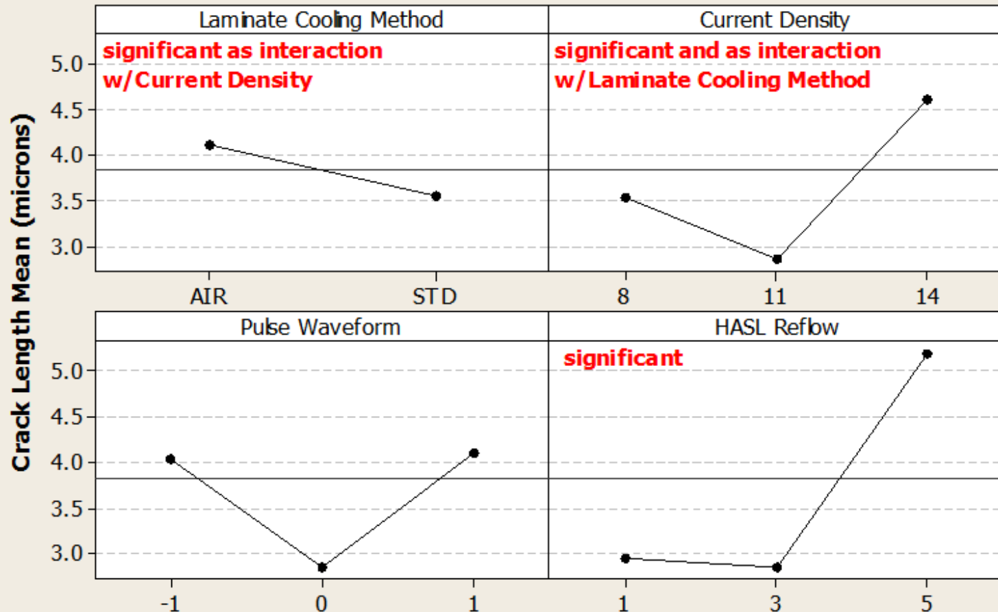
Main Effects Plot: 635 u PTH coupons
