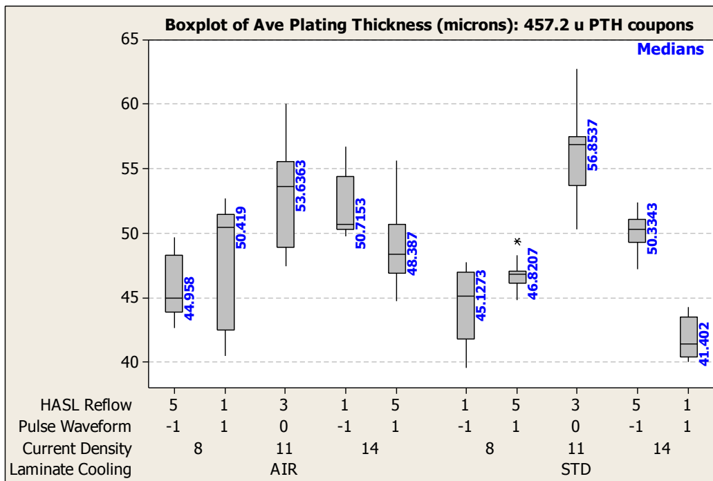
Figure 7 - Box Plot of Average Plating Thickness (457.2 \mu m PTH coupons)
