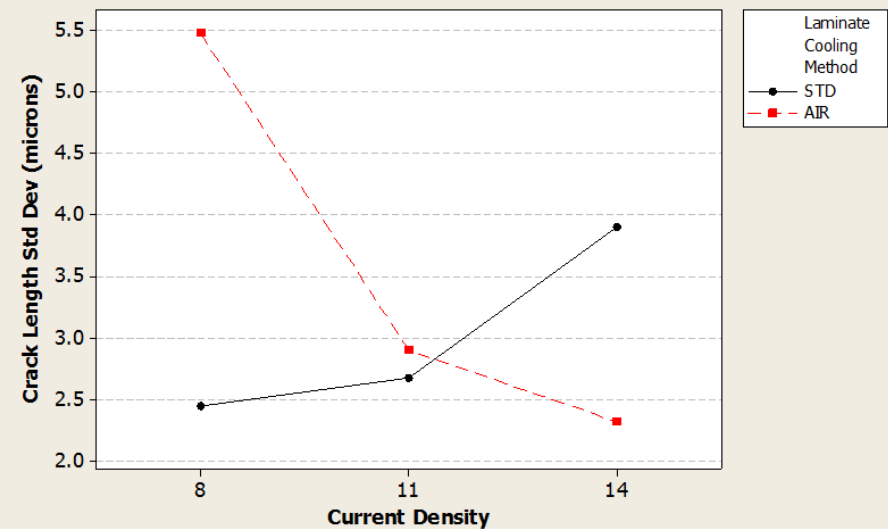
Interaction Plot for Crack Length Std Dev: buried via coupons
