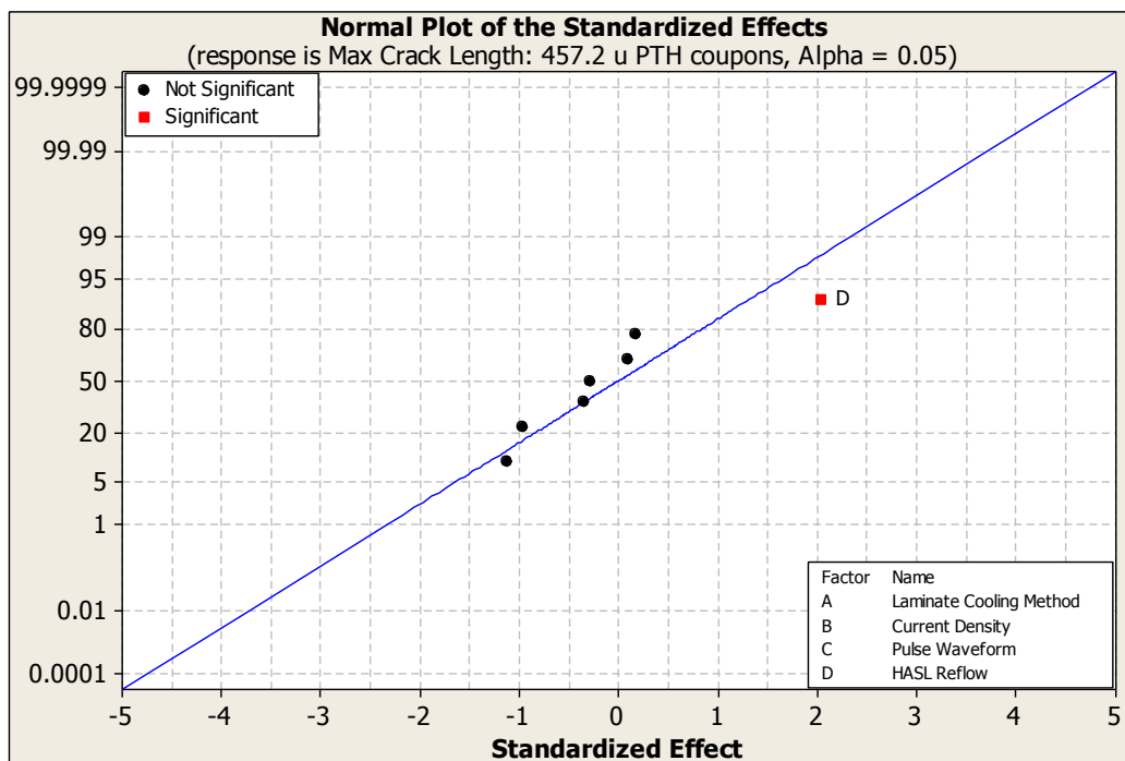
Figure 10 - Normal Probability Plot of the Effects: Maximum Crack Length (457.2 \mu m PTH coupons)
