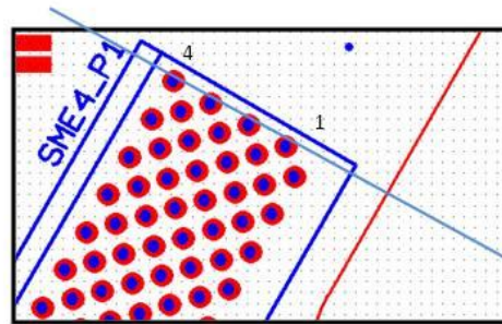
Coupon 1 (4 Locations- 635 \mu\text{m} (.025") PTH )
