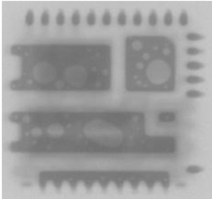
Regular QFN
