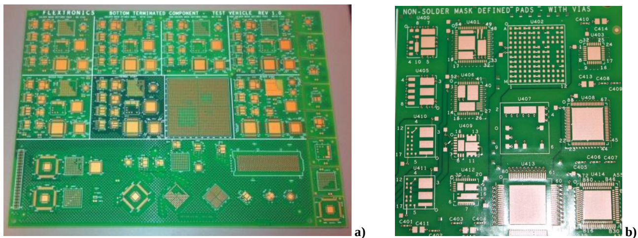
Figure 1 - Company Bottom Terminated Component Test Vehicle a) Topside b) Various BTC Pad Design.
