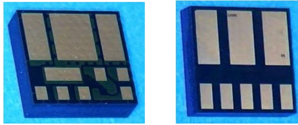
Figure 5 - LGA Images_ Non-identical Pad Size for Signal and Ground Pins.
