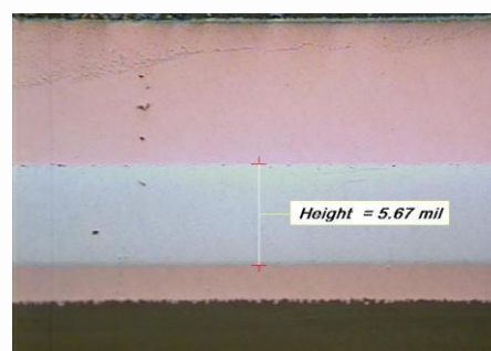
Pre-tinned QFN Joint
