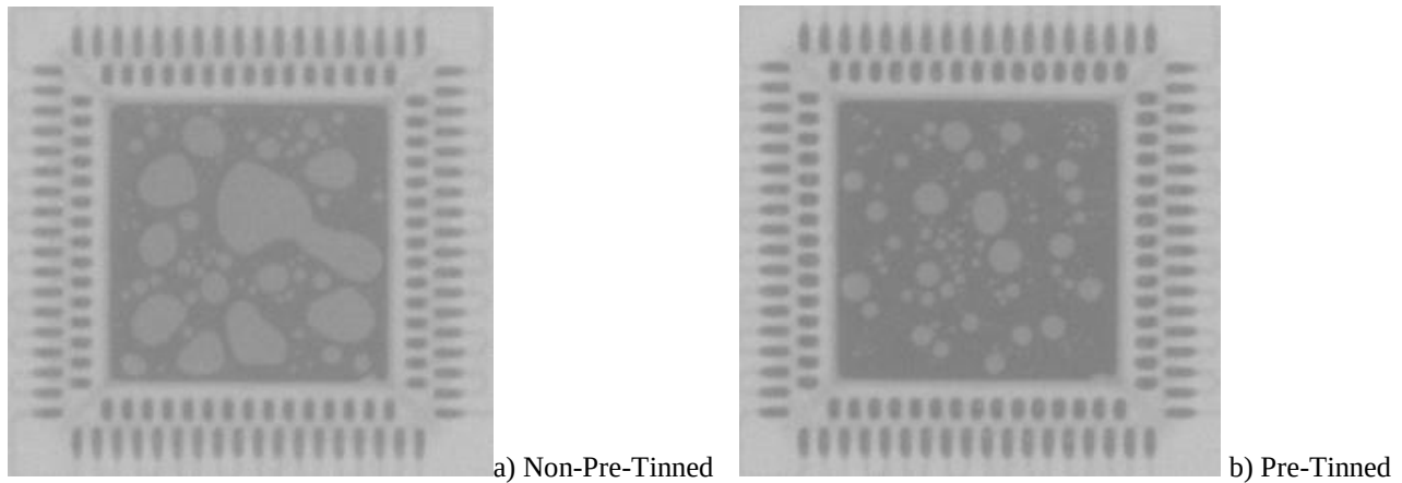
Figure 9 - X-Ray Images of QFN132 Solder Joint Assembled with Non-Pre-Tinned Component vs. Pre-Tinned Component.
