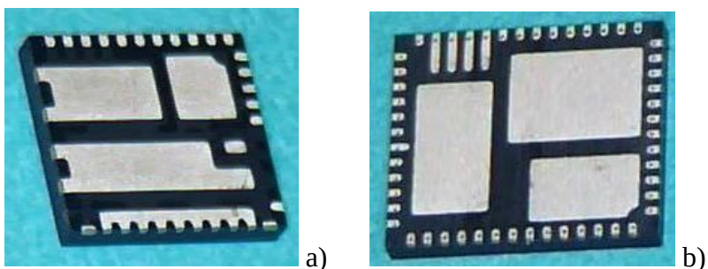
Figure 3 - Non-symmetrical QFN Component Images.
