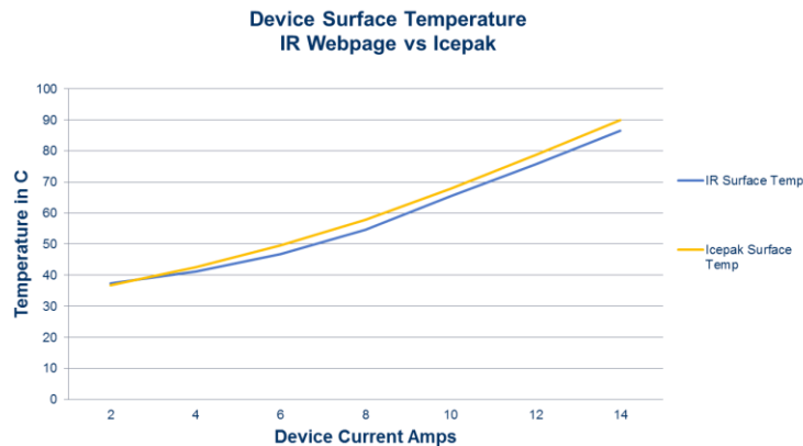
Figure 19 - Temperature Behavior from Model versus Device Supplier Data
