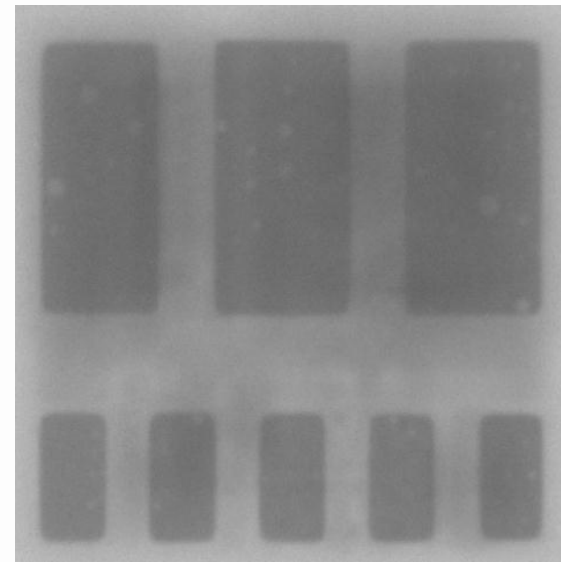
Pre-tinned LGA
