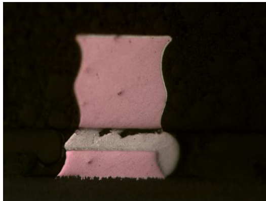
Figure 14 - Cross Section Images after 3000 Cycles for QFN52_ Non-Pre-tinned. Crack was usually seen at the component side.
