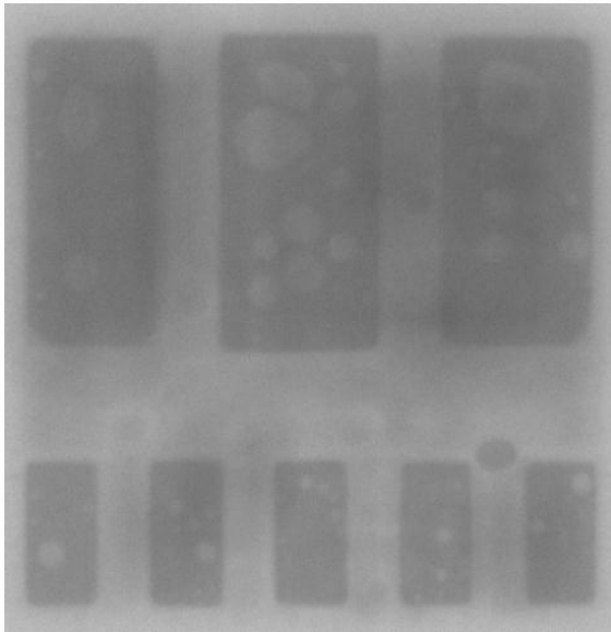
Regular LGA
