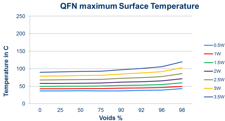
Figure 20 - Solder Voiding Impact on the Device Temperature at Different Power Dissipation
