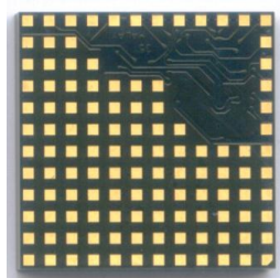
Figure 4 - LGA Images_ Identical Pad Size for Signal and Ground Pins.
