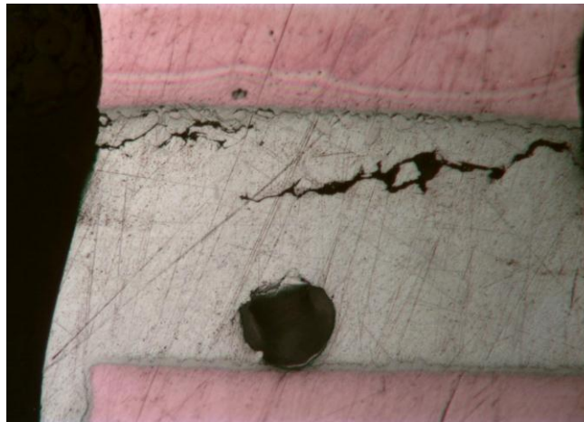
Figure 15 - Cross Section Images after 3000 Cycles for QFN88_ Pre-tinned Component. Cracks were seen at the component side and through the solder joint.
