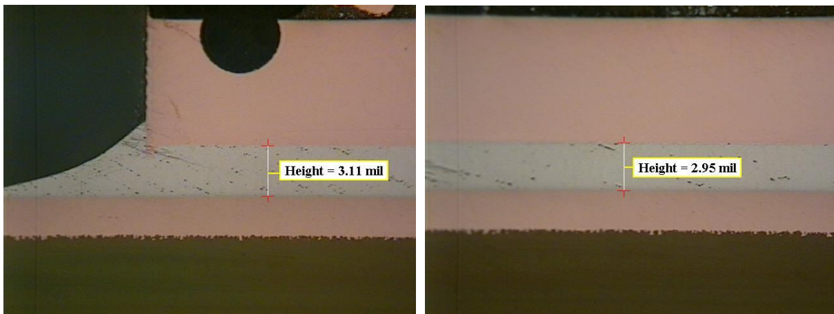
Figure 10 - Cross Section Images of a QFN component at t=0_ Non-Pre-tinned Component
