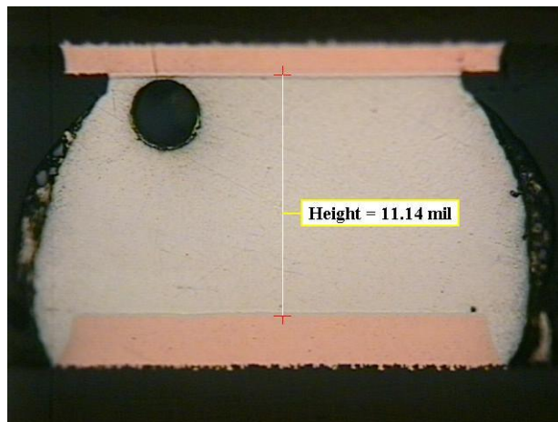
Figure 12 - Cross Section Images of BGA Component after Reflow
