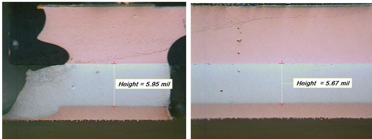
Figure 11 - Cross Section Images of a QFN Component after Reflow_ Using Pre-tinned Components
