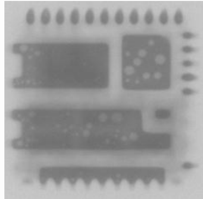
Pre-tinned QFN
