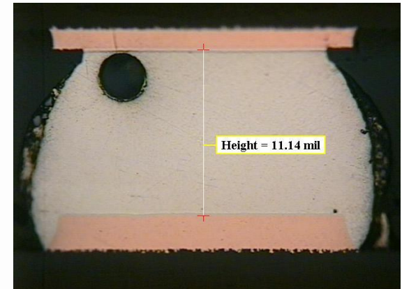
BGA Solder Joint
