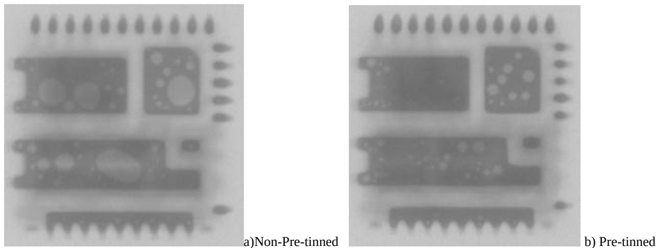
Figure 8 - X-Ray Images of QFN 3550 Solder Joint Assembled with Non-Pre-tinned Component vs. Pre-tinned Component.
