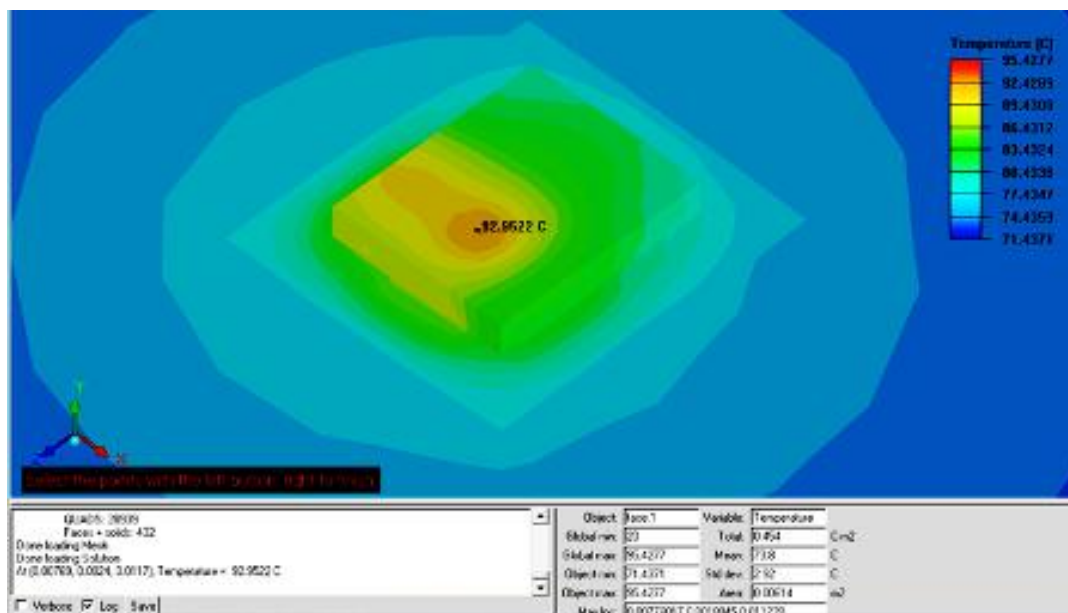
Figure 21 - Simulator Results for a Scenario of 75% Voids and 3.5W
