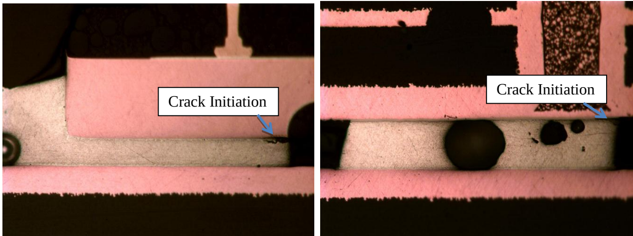
Figure 13 - Cross Section Images of BTC Component after 1000 Cycle.
