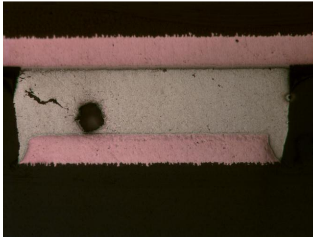
Figure 16 - Cross Section Images of QFN Component After 3000 Cycles. Crack initiated at the solder joint, not at the void area.
