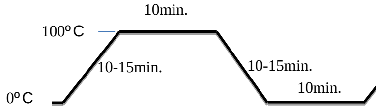
Figure 6 - Thermal Cycle Temperature Profile – 0 to 100 degrees C
