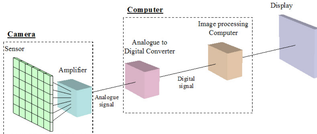
Figure 3 – Analogue Detector Based x-ray System Schematic
