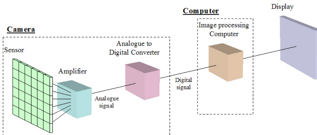
Figure 4 – Digital Detector Based x-ray System Schematic
