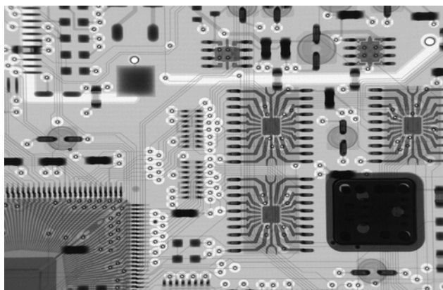
Figure 2 - 1.3 Mpixel Digital Intensifier X-ray Image of PCB in Figure 1
