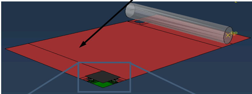
Global Modell 2D PCB = Composite Shell
