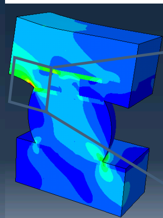
Mises Stress Sub Model
