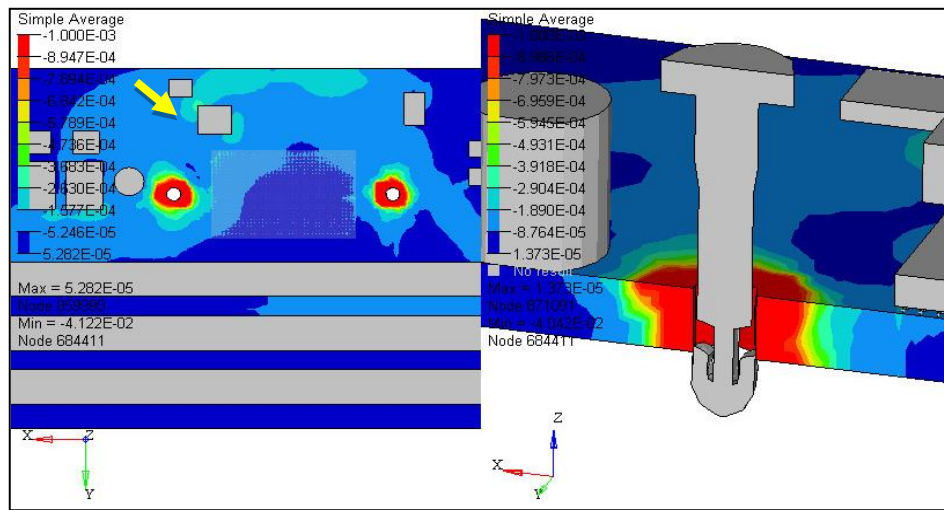
Figure 8. Max. Principal Strain (manual)
