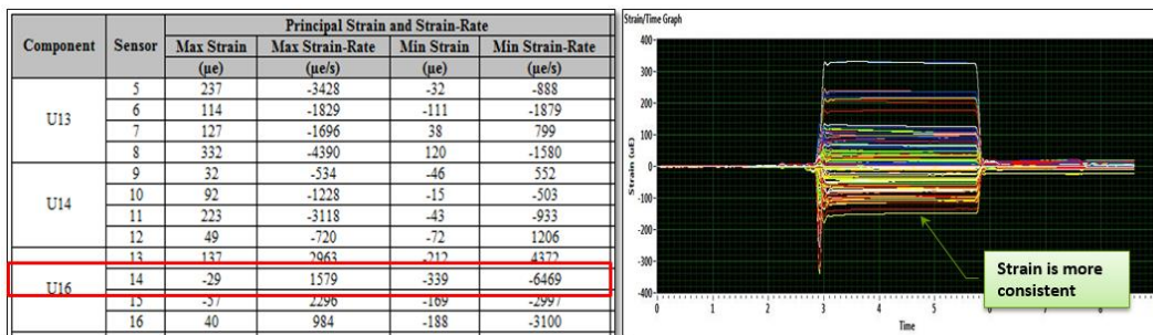
Figure 5. Max. Strain & Graph of Automated Assembly
