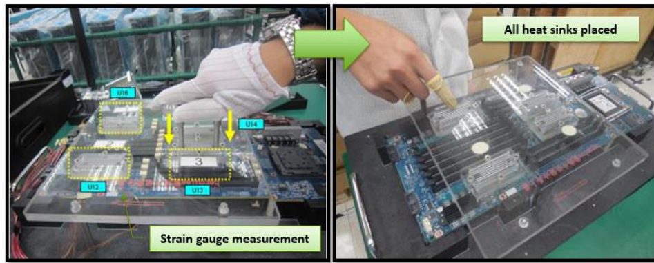
Figure 1. Strain gauge on manual assembly set-up
