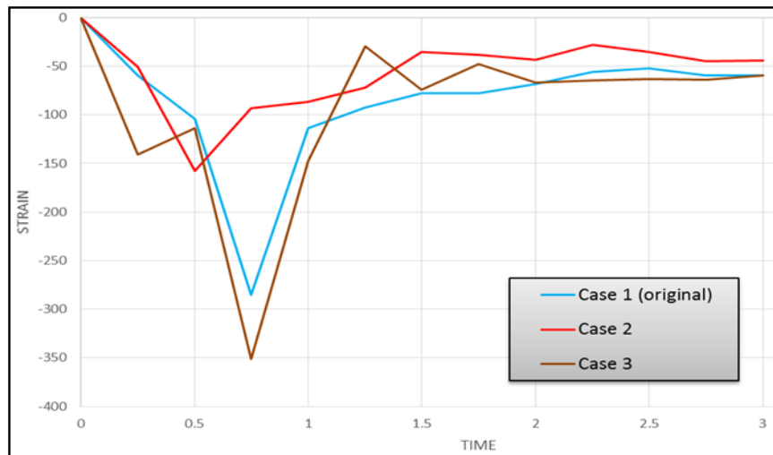
Figure 11. Max. Strain Graph (BGA location change)
