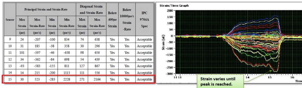
Figure 4. Max. Strain & Graph of Manual Assembly
