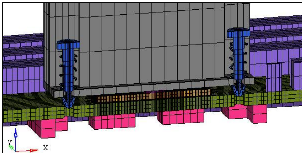
Figure 3. FEA model
