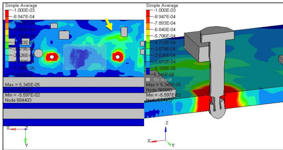
Figure 10. Max. Principal Strain (automated)
