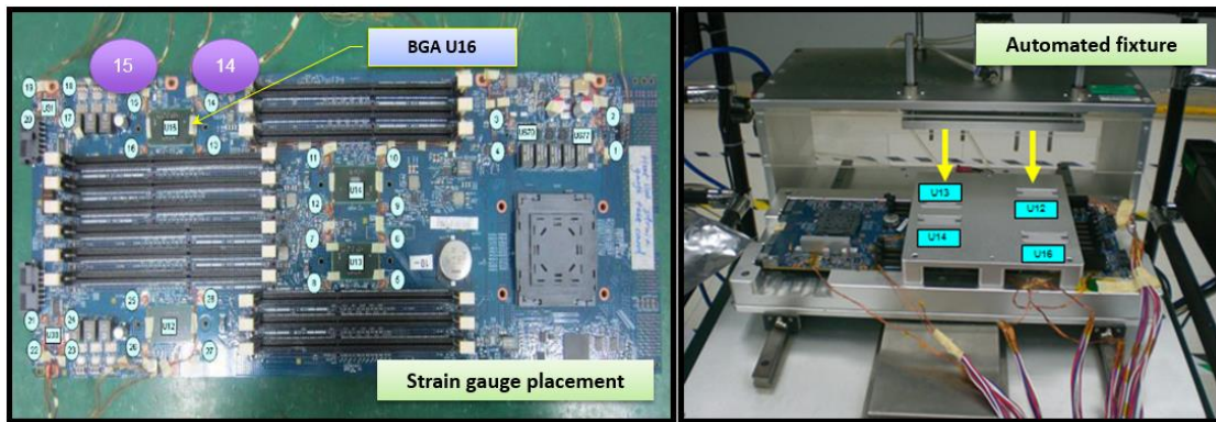
Figure 2. Strain gauge on automated assembly
