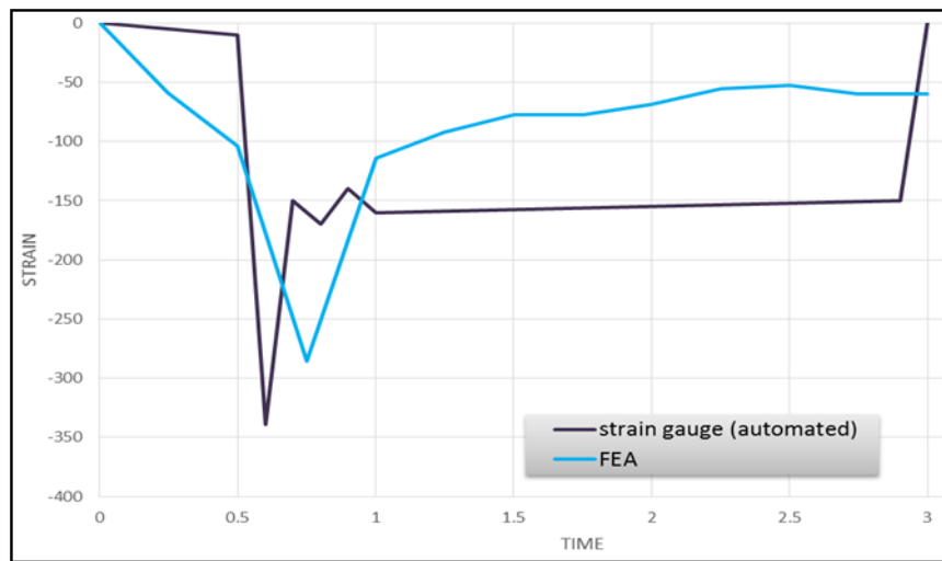
Figure 9. Max. Strain Graph (comparison for automated process)
