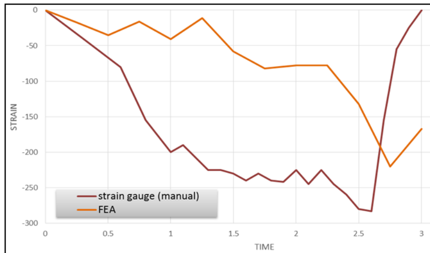
Figure 7. Max. Strain Graph (comparison for manual process)
