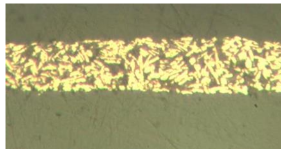
Effect of photonic sintering
