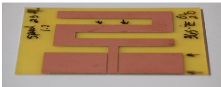
Printed Cu Antenna on FR-4
