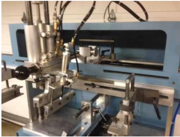
Figure 1. Screen printing equipment can range from manual to semi-automatic (pictured) to fully automatic.
