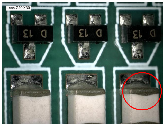
Figure 10: Alloy B – Peak of 240°C at 30 sec TAL Cold Solder
