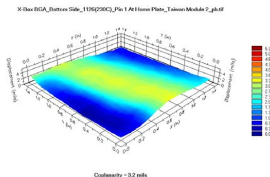
Figure # 15: Thermoiré image of the bottom side of the BGA showing a coplanarity of 3.2 mils along all BGA Ball at 230°C
