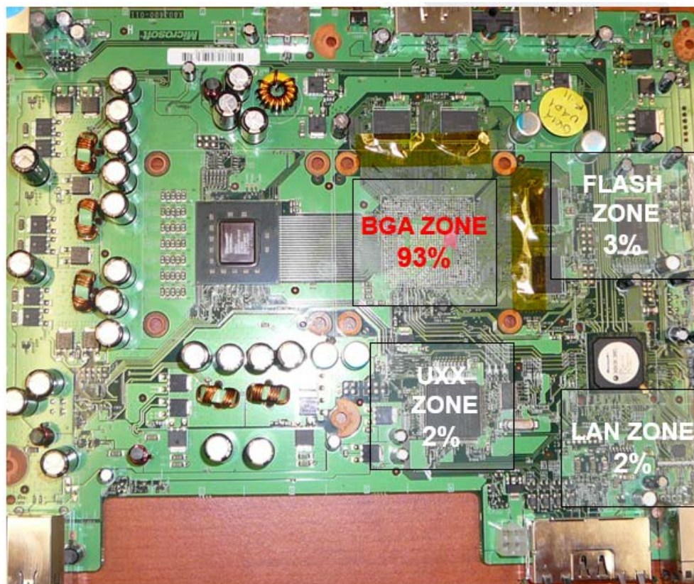
BGA Rework defect concentration diagram
