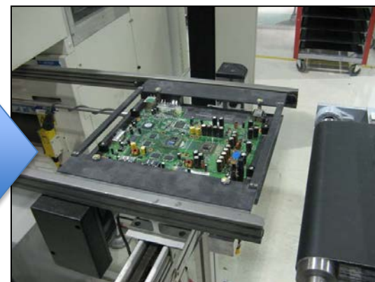
Exit area (Pallet in Down position)
