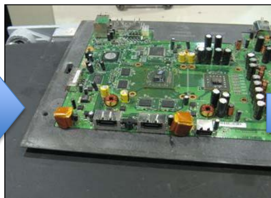
Place extra covers for sensitive TH connector
