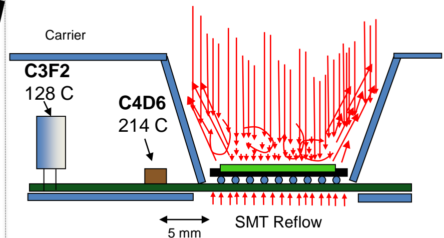
Selective Reflow Rework Process
