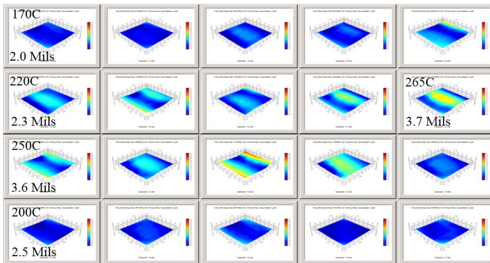
Figure # 16: Thermoiré images at every 10 degrees showing BGA behavior under thermal stress
