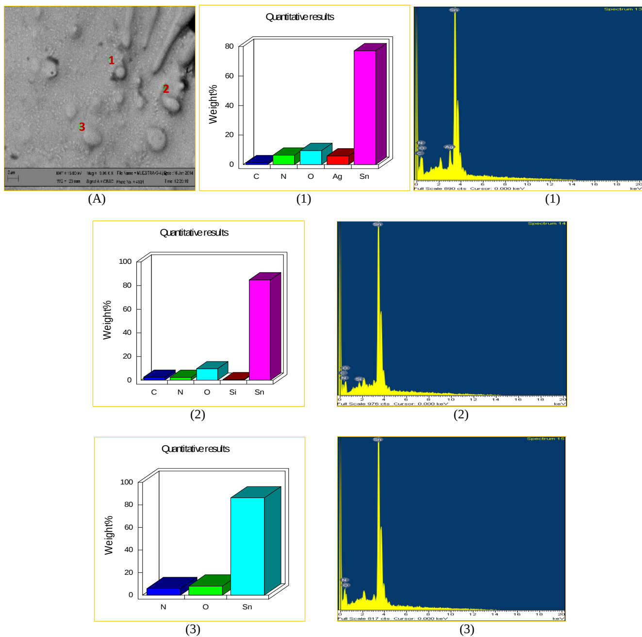
Figure 15. (A) shows three red numbers representing the punctual areas. (1) corresponds to the analyzed point 1, (2) to the analyzed point 2, and (3) to the analyzed point 3. The sample comes from 16 hrs test and DI water
