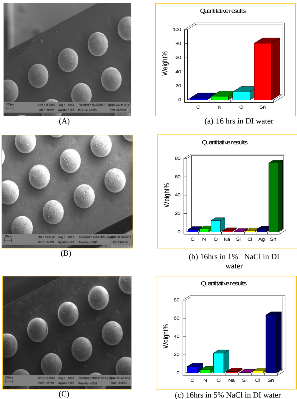
Figure 10. DOE 2. SEM Analysis Influence of NaCl in several conditions
