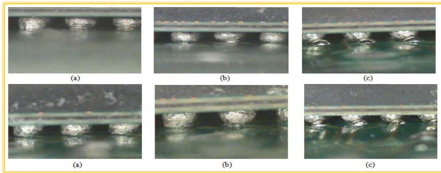
Figure 4. DOE 1 Results: (a) Components at 4 hrs of steaming, (b) Components at 8 hrs of steaming, and (c) Components at 16 hrs of steaming, the components are misplaced due to number of HiP's.
