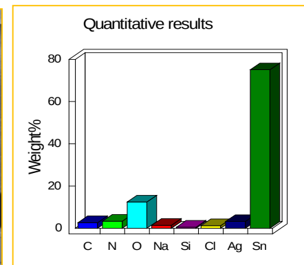
(b) 16hrs in 1% NaCl in DI water
