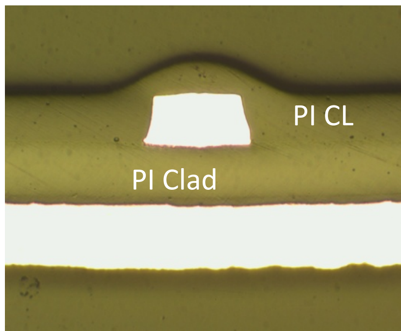
Coverlay
