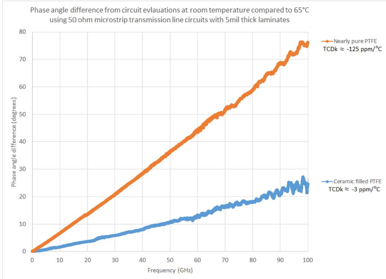
Figure 3. Phase angle testing of 8" (203mm) long 50 ohm microstrip transmission line circuits, comparing room temperature conditions to operating at 65°C.
