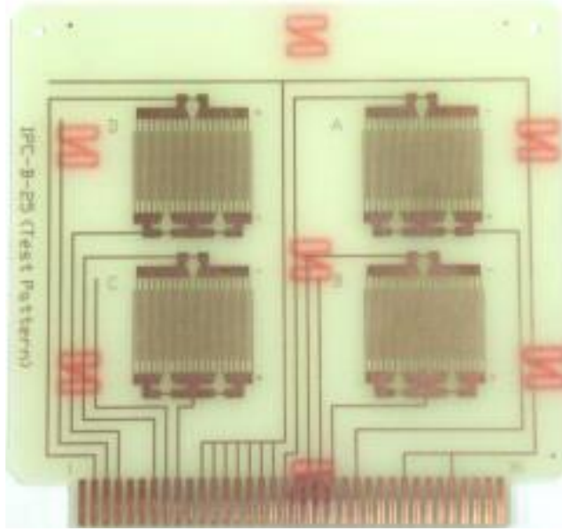
Figure 3: IPC-B-25 test board (E pattern)
