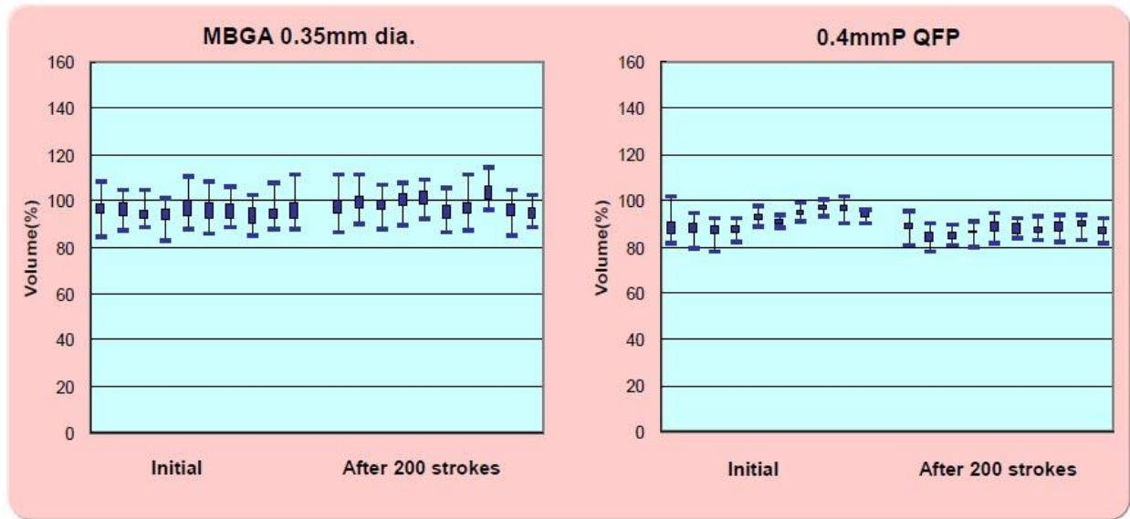
Figure 16: Crack-free Paste A printing SPI data for 0.35mm diameter BGA pads and 0.4mm pitch QFP pads.
