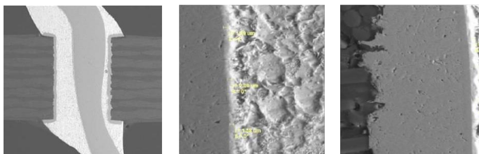
Figure 4 Sample#2 Cross sectional analysis
