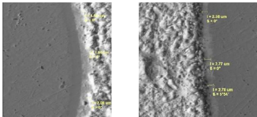
Figure 11 Sample#3 Cross sectional analysis
