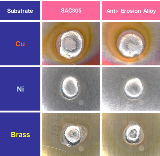
Figure 11: Wetting results of SAC305 and Sn0.3Ag0.7Cu0.04Co on different substrates (Copper, Nickel and Brass).
