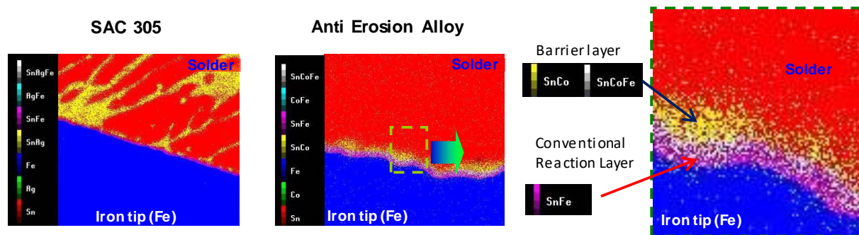
Figure 15: EPMA (Electron probe micro-analysis) of boundaries between solder and iron tip. (Sn3Ag0.5Cu compared with Sn0.3Ag0.7Cu0.04Co alloy)
