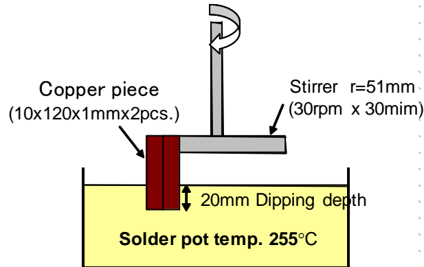
Figure 3: Copper Plate Erosion Test Schematic
