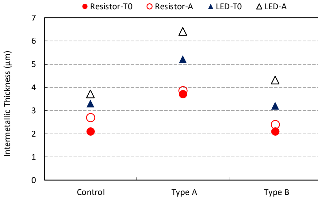
Figure 17: Board Side Intermetallic Thicknesses for different components (Resistor and LED) under different conditions (Control- SnAgCu 1 st pass, A- SnAgCu 1 st pass + SnAgCu rework, B- SnAgCu 1 st pass + Sn0.3Ag0.7Cu0.04Co rework) before and after thermal cycling
