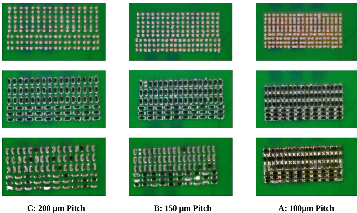
Figure 3 – Optical Picture: After Print (top), After Placement (center), and After Reflow (bottom)
