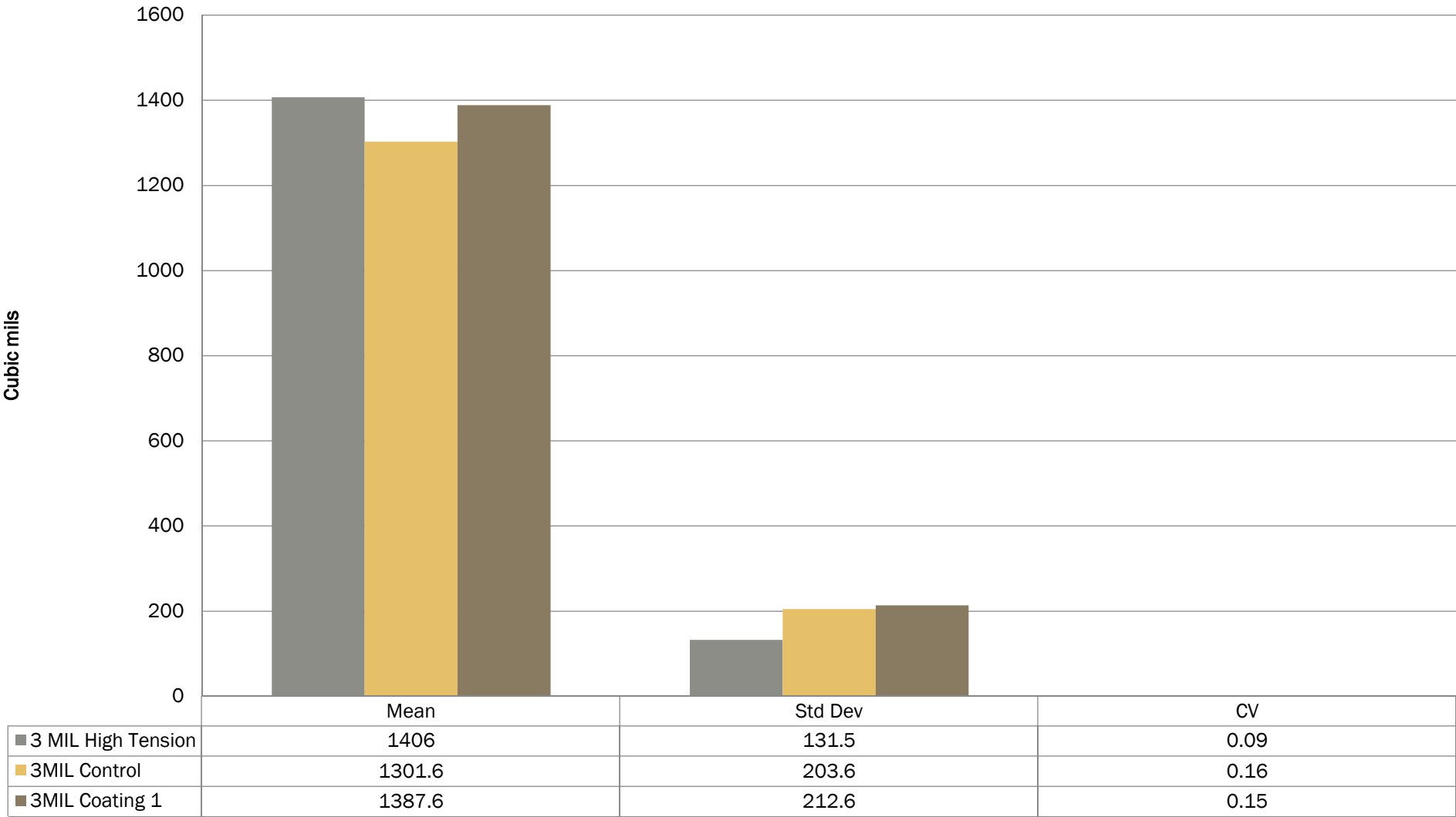
Solder Paste Volume 0402 Component-3 mil stencil
