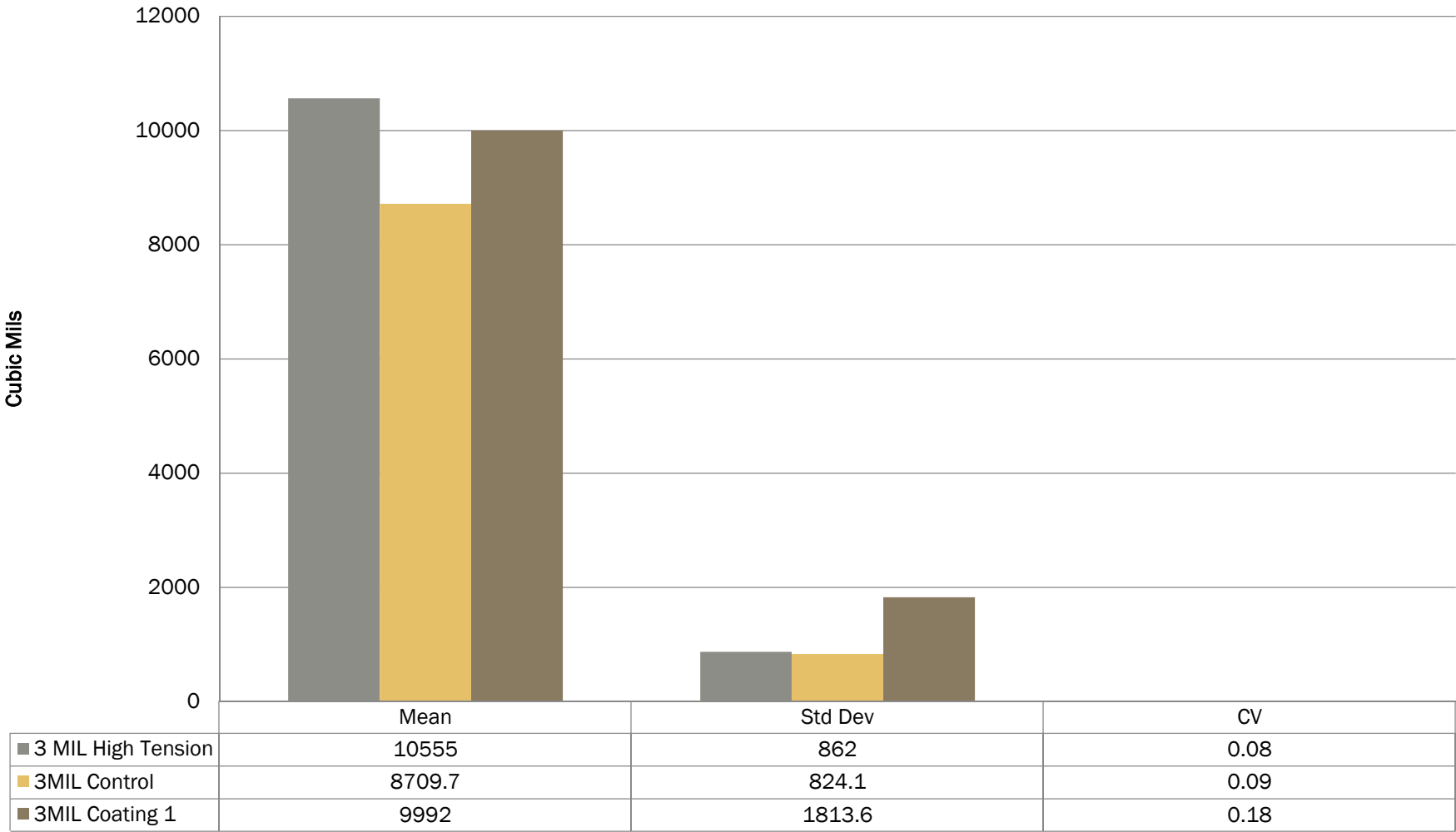
Solder Paste Volume 1206 Component- 3 mil stencil
