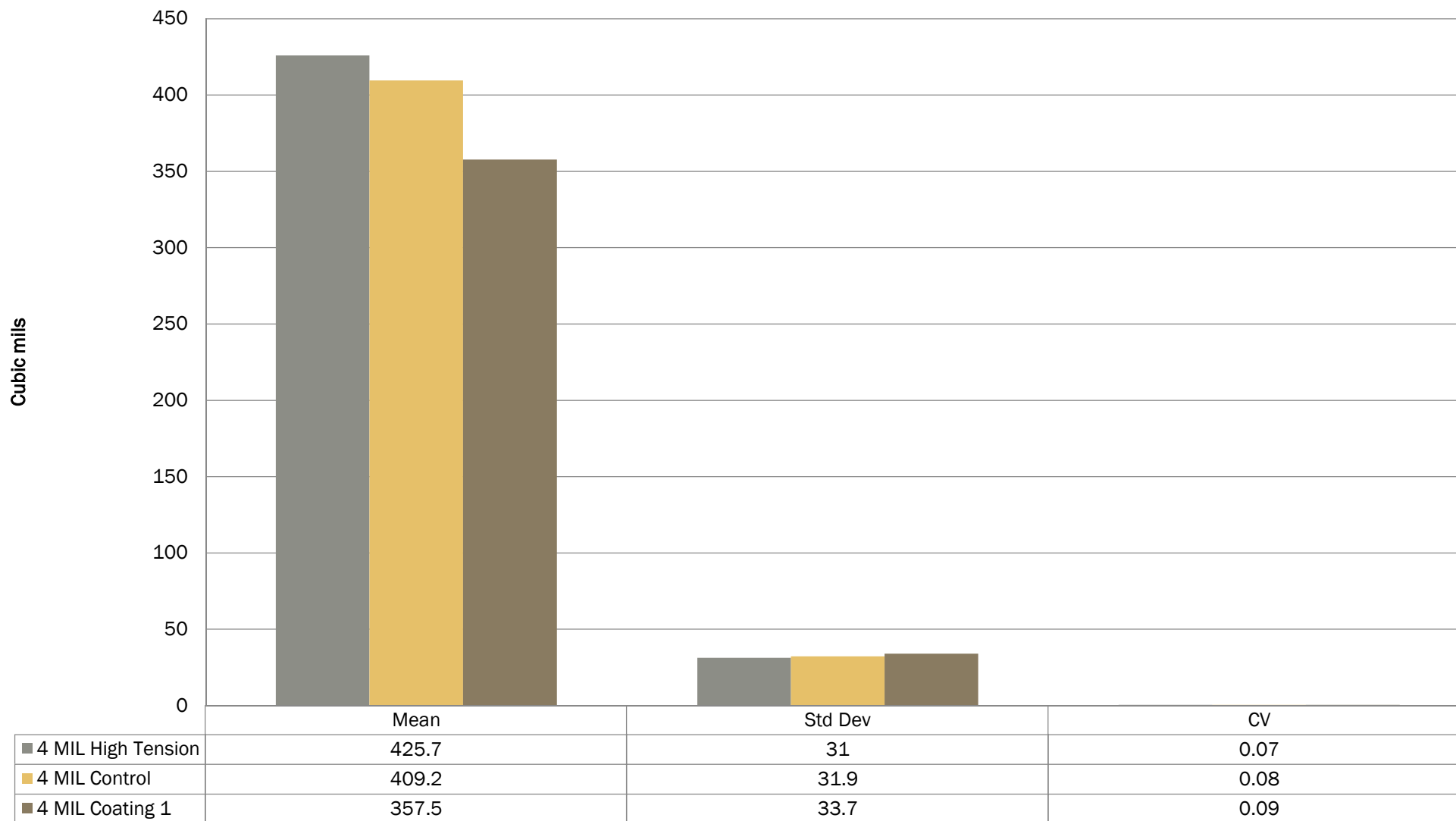
Solder Paste Volume 0201 Component-4 mil stencil
