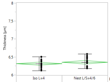
Figure 9 - Achieved Cu Thickness distribution on a 600x600mm Panel
