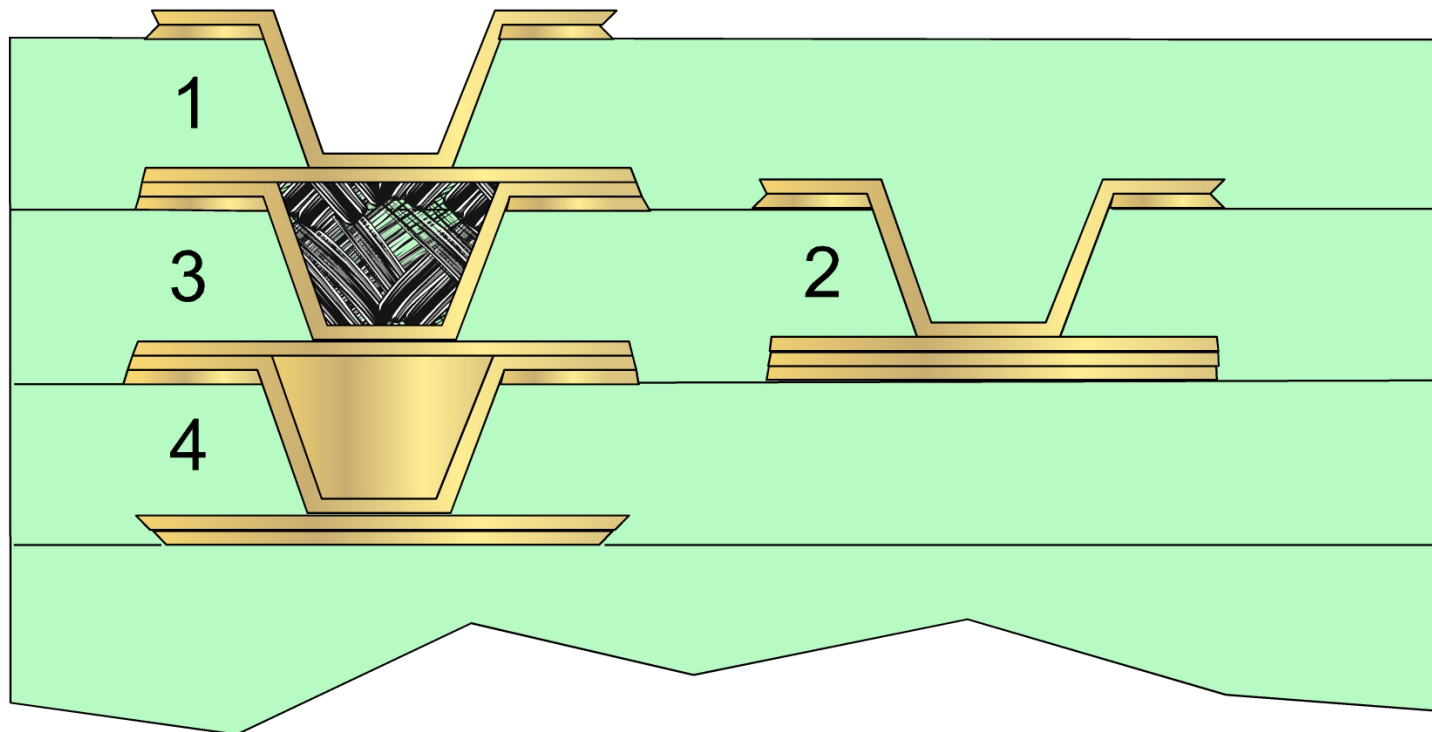
Ranking of Microvias by Fill Type
