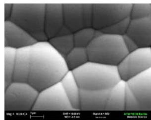
Figure 3: Pure Pd deposition (0.15µm) over nickel, showing some nano-roughness on the surface. and smooth surface.
