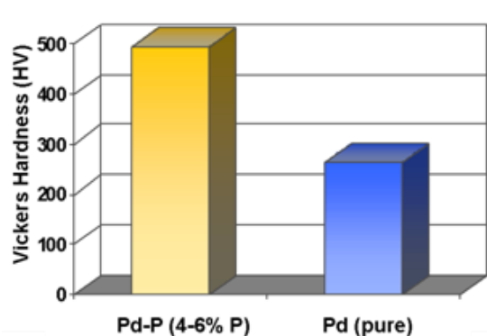
Figure 1: Comparison of hardness of palladium-phosphorus and pure palladium autocatalytic deposits.
