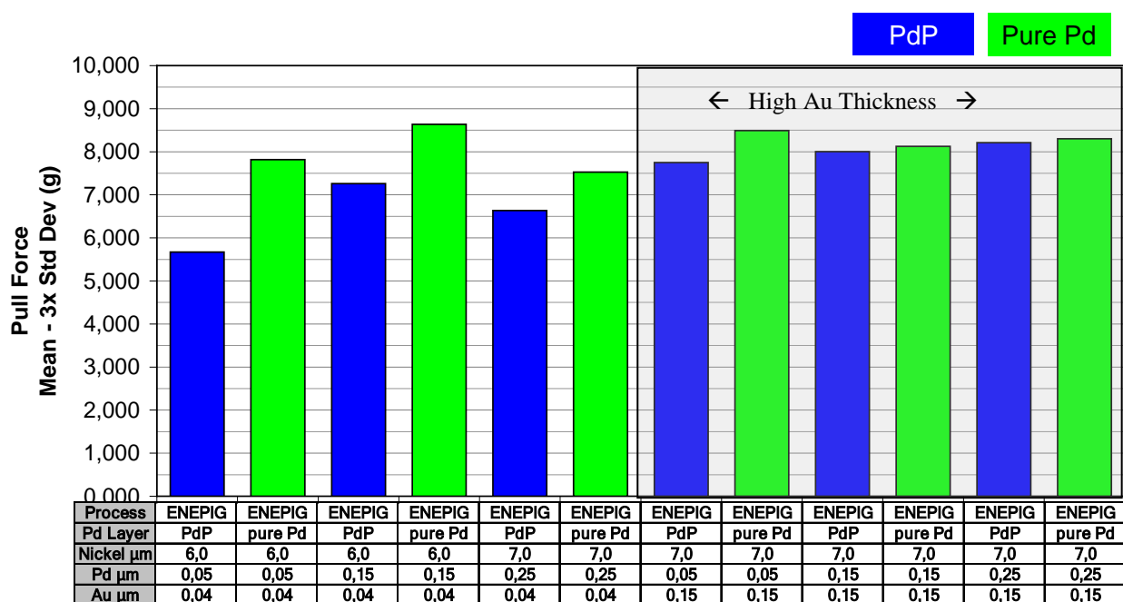
Figure 7: Comparison of gold wire bond pull test results for ENEPIG (with PdP) vs. ENEPIG (with pure Pd) with varying thickness of Ni, Pd and Au
