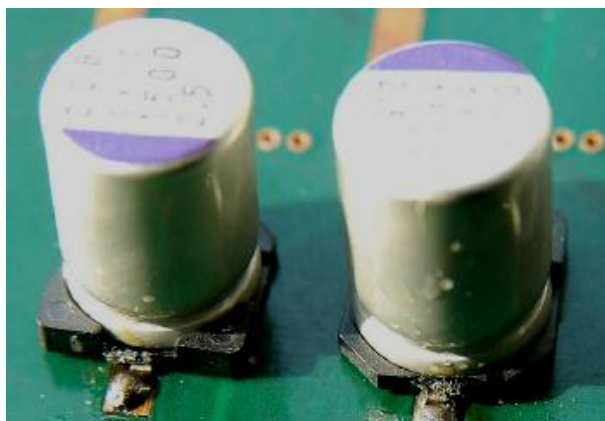
SMT Electrolytic
