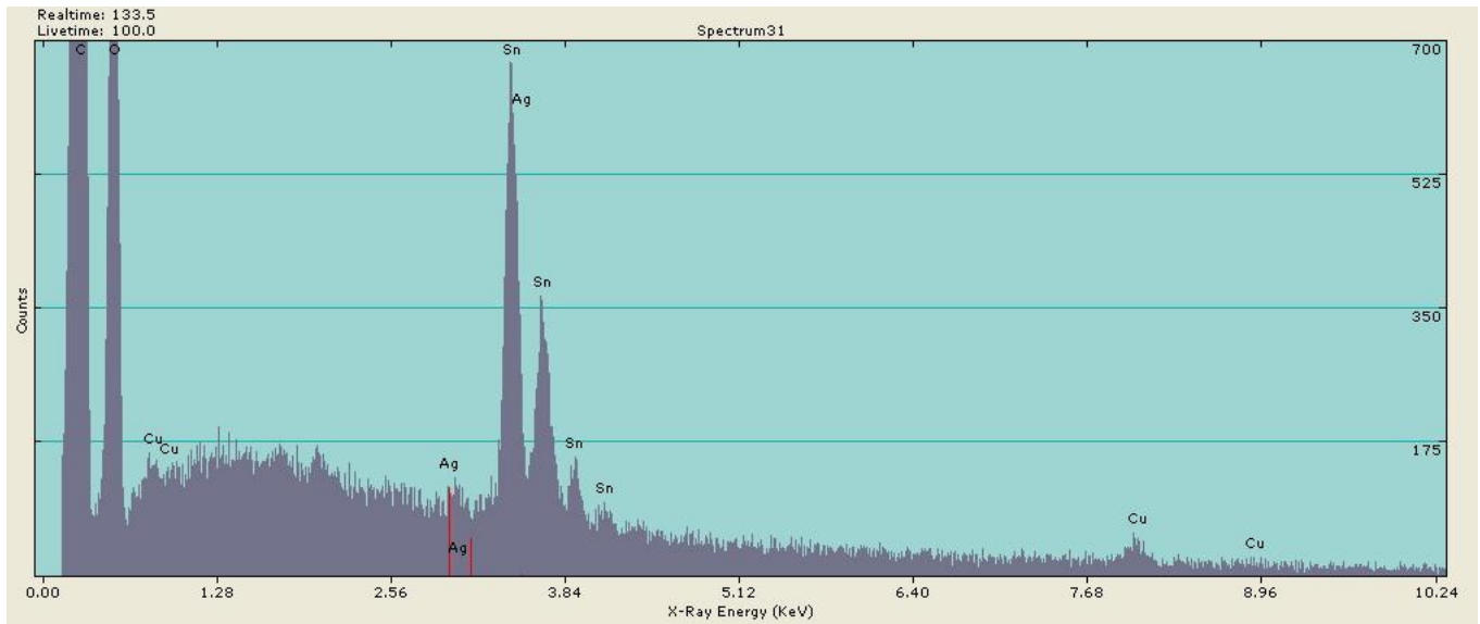
Figure 10: EDX Scan of Surface Metal Haloing Around the Solder Deposit.
