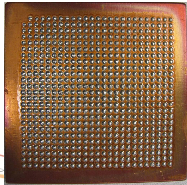
Post Reflow
