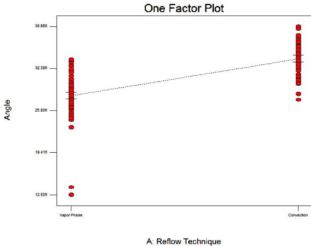
Figure 14: ANOVA One Factor Plot of Wetting Angles Between Vapor Phase and Convection Reflow.
