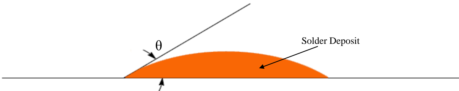
Figure 1: Example of Wetting Angle
