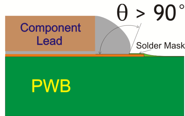
Wetting Angle Greater than 90^\circ but Over Solder Resist
