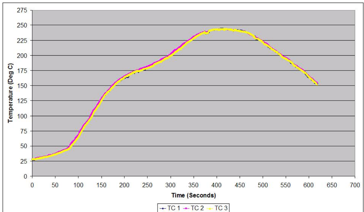
Figure 6: Pb Free Convection Reflow Thermal Profile used.
