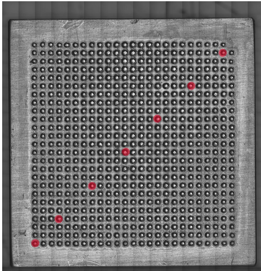
Figure 11: The 7 Solder Deposits Examined on Each Cu Block Sample. Red Dots show measurement locations.
