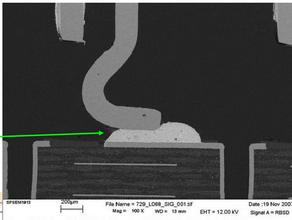
Wetting Angle Greater than 90^\circ but Over Edge of Solderable Area
