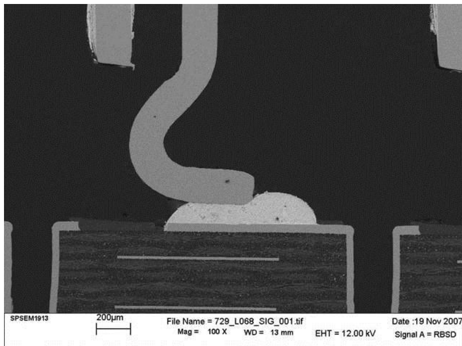
Figure 3: Example of non-wet Solder Joint.
