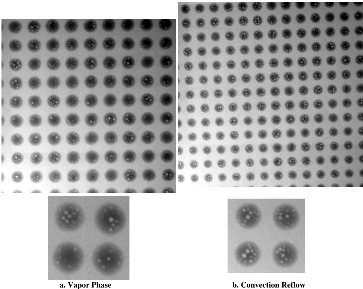
Figure 15: Comparison of X-ray Inspection of Solder Bumps between Vapor Phase and Convection.
