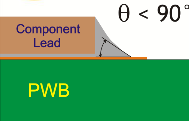
Wetting Angle Less than 90^\circ
