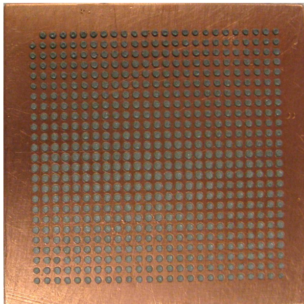
Solder Deposit
