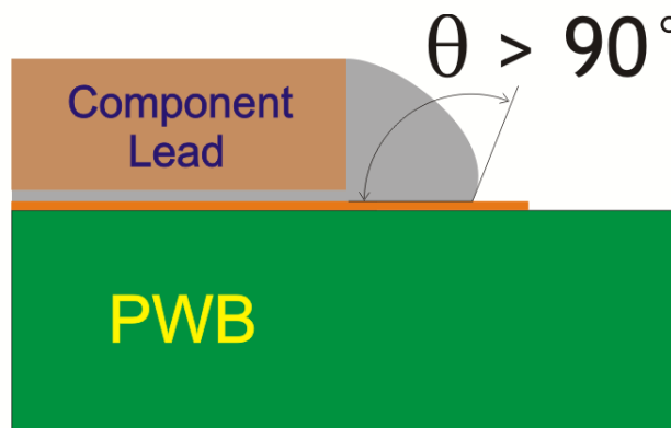
Wetting Angle Greater than 90^\circ but Over Edge of Solderable Area
