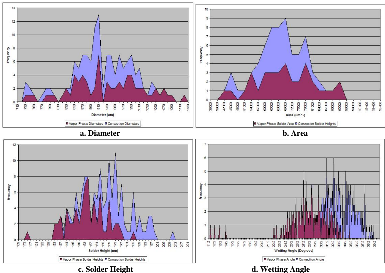
Figure 13: Histograms of Various Measurements Taken from the Different Solder Bumps.
