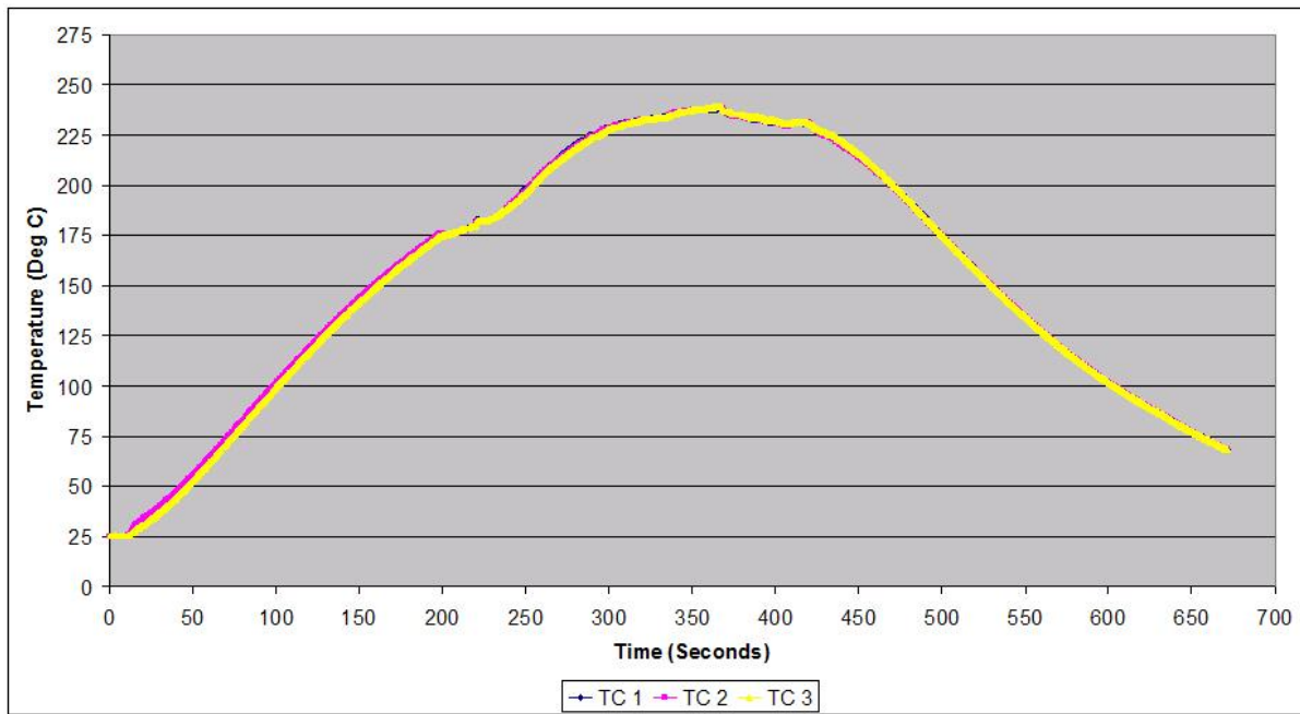
Figure 5: Pb Free Vapor Phase Thermal Profile used.
