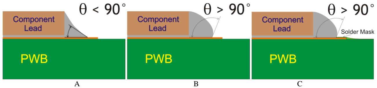
Figure 2: Acceptable wetting angles for solder joints are covered in IPC-A-610. Pictures A shows wetting angle less than 90^\circ . Picture B shows a wetting angle greater than 90^\circ formed over the edge of the solderable termination area. Picture C shows a wetting angle greater than 90^\circ formed over solder resist (Bielick, 2010).
