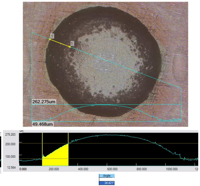
d. Wetting Angle = 34.421°
