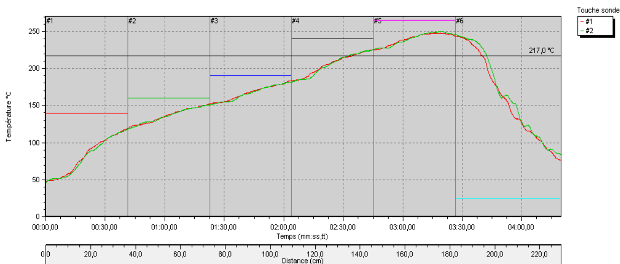
Figure 2: Convection thermal profile
