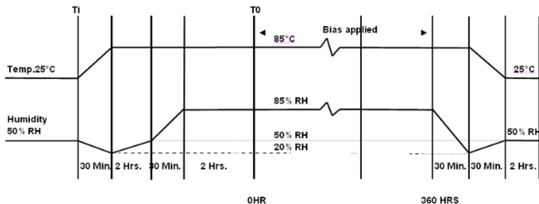
Temperature - Humidity Curve "Condensation-Free"
