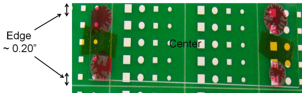
Figure 8 - Picture showing the edges and center of the glass slides where flux removal effectiveness was rated
