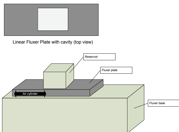
Linear Fluxer in Closed Position
